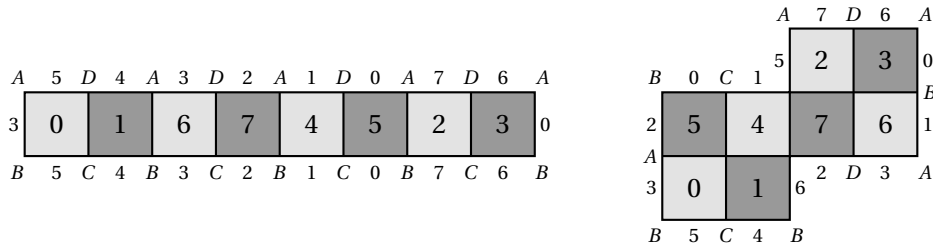
FIGURE 4. These two ways to unfold the square-tiled cyclic cover M_4(1,3,2,2) represent decompositions into horizontal and into vertical cylinders
