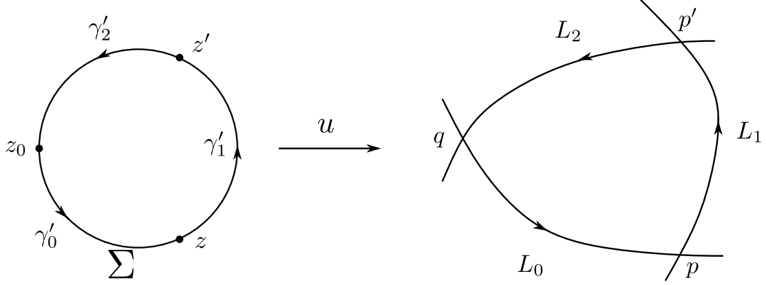
Figure 4.4 – Product in Floer cohomology
