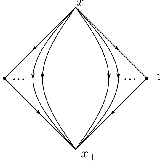
Figure 2.1 – Compactification of \widehat{\mathcal{M}}(x_-, x_+; f, X) .
