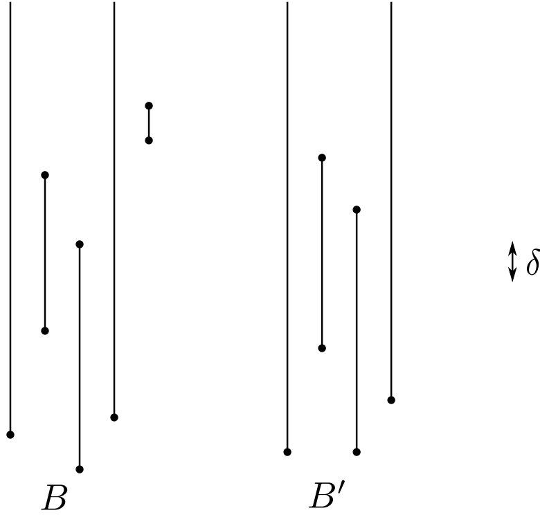
Figure 3.1 – Two barcodes B and B' such that d_{bottle}(B, B') \leq \delta
