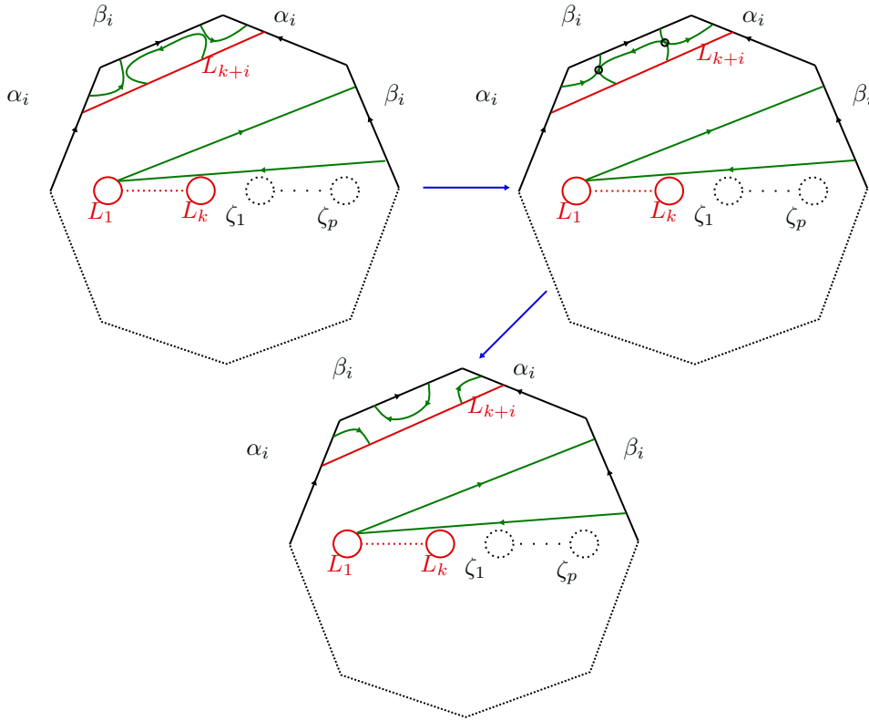
Figure 2.8: Homotopy between b_i^{-1}a_ib_i and the constant path
