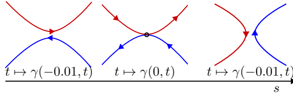
Figure 2.4: The homotopy \gamma(s, t) as seen on \mathbb{C} .
