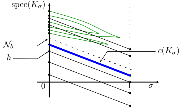
Figure 10: The bifurcation diagram of the deformation K_\sigma .
