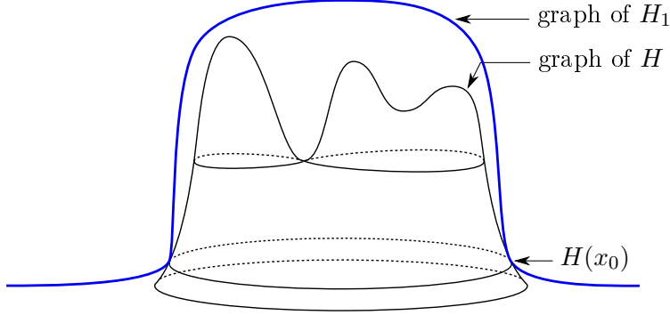
Figure 8: (Proof of Claim 30) construction of H_1 \geq H with c(H_1) = \mathcal{N}_b
