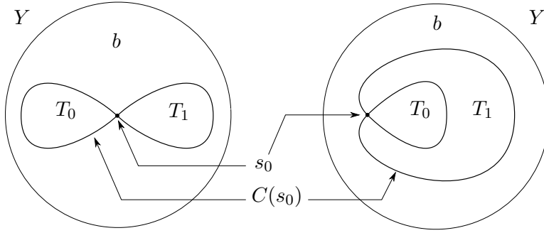
Figure 5: Notations Y, s_0, C(s_0), b, T_0, T_1 : the two cases
