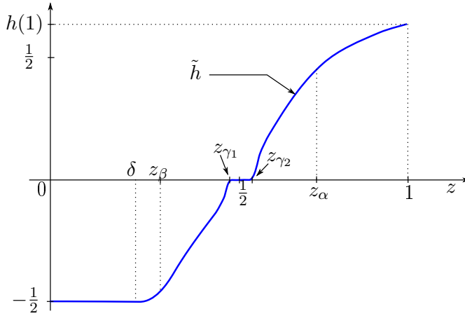
Figure 15: Graph of \tilde{h} .
