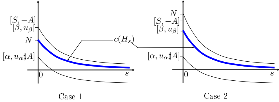
Figure 16: The bifurcation diagrams of H_s . Each curve represents the value of the action \mathcal{A}_{H_s} corresponding to the indicated point.
