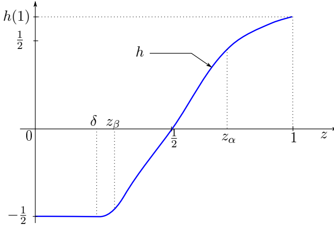
Figure 14: Graph of h .
