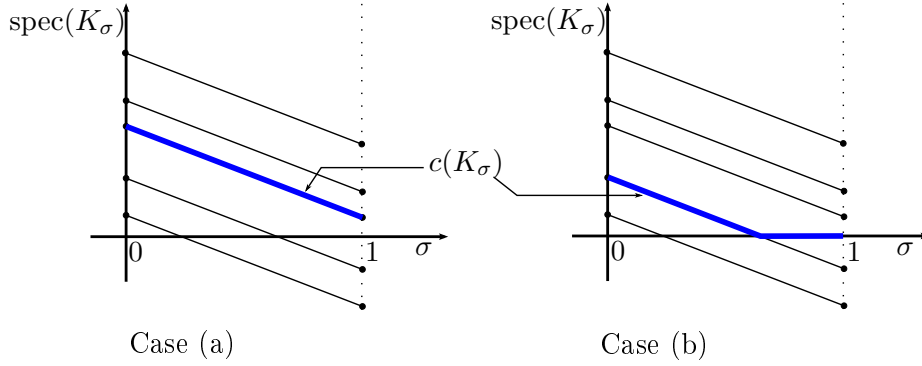
Figure 6: Bifurcation diagram for the spectrum of the deformation K_\sigma : (a) represents the case H(s_0) + c(\bar{H}_{T_0} + \bar{H}_{T_1}) > 0 and (b) the opposite case.
