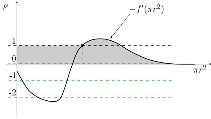
Figure 3: The fixed point correspond to intersections of the graph \rho = -f' with the horizontal lines “ \rho = \text{integer constant} ”. The action of the thick black dot is the area of the grey region. This thick black dot corresponds to the thick black dot on Figure 2.
