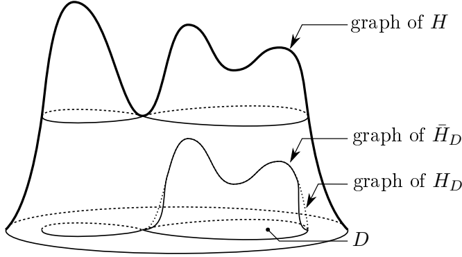
Figure 4: Graphs of H, H_D, \bar{H}_D
