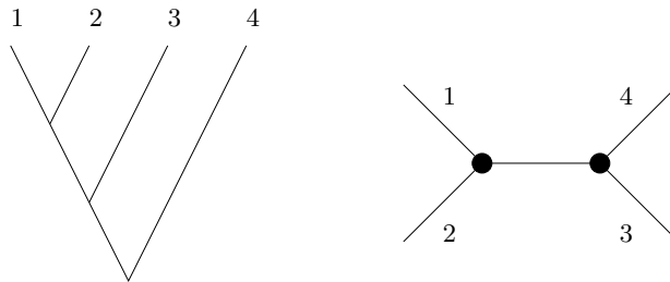
Figure 3: A tree and its associated admissible graph
