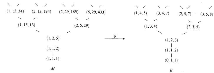
FIGURE 2. THE MARKOFF TREE AND THE EUCLID TREE
