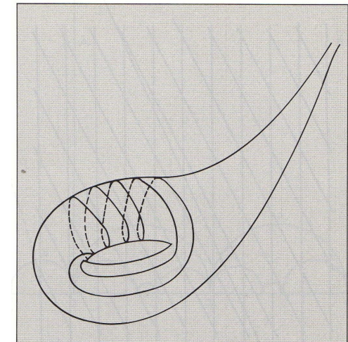
Figure 1. A simple curve on the punctured torus.
