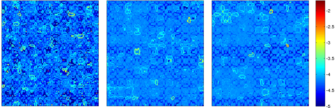
FIGURE 12. Simulations of invariant measures \mu_{\mathbf{T}^2}^{(g_1)^N} on the grids E_N , with N = 2^k , k = 10, 14, 15 (from left to right and top to bottom).
