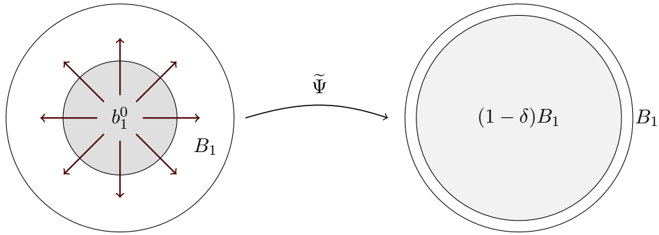
FIGURE 4.1. L'application \tilde{\Psi}
