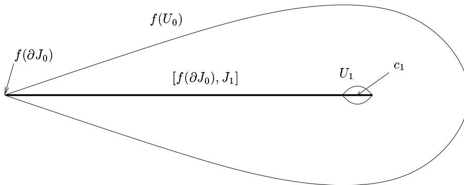
FIGURE 4. Inside f(U_0) .
