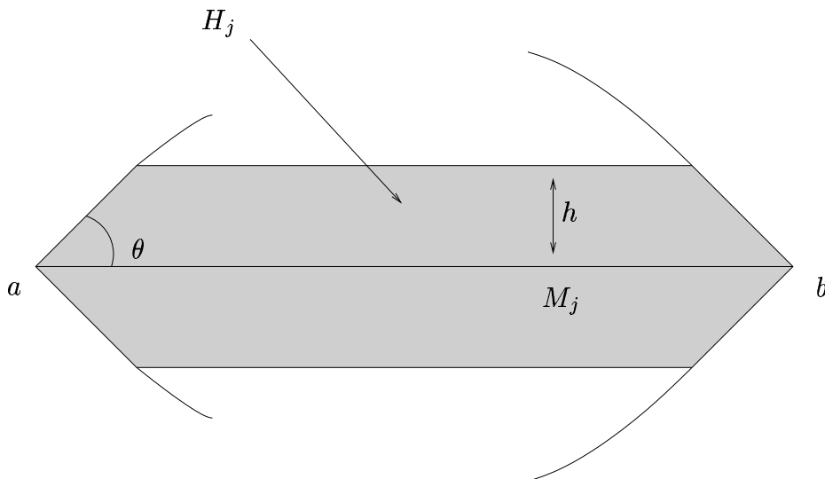
FIGURE 6. A hexagonal Markov piece.
