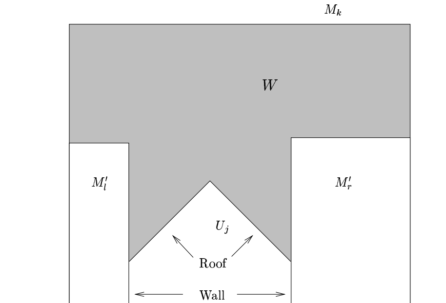
FIGURE 7. Inside a Markov piece
