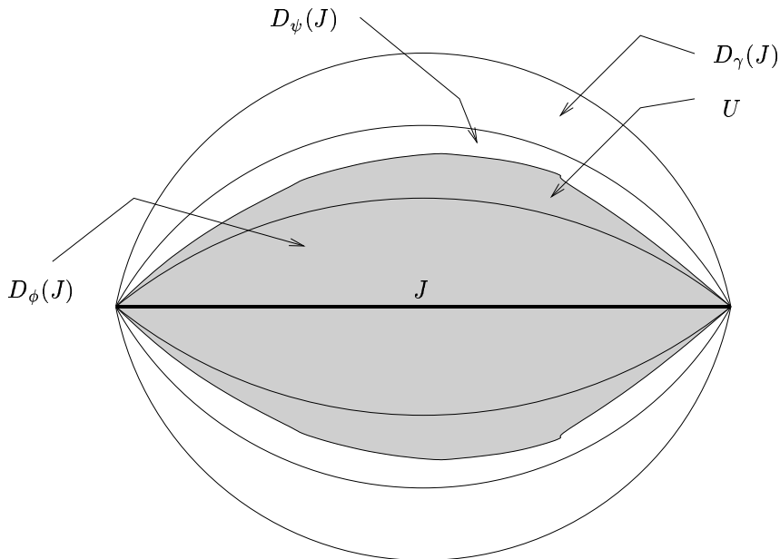
FIGURE 3. Geometric domains.
