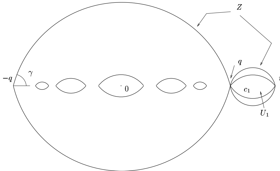
FIGURE 5. Set Z and the puzzle
