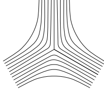
FIGURE 1. A 3-pronged singularity.
