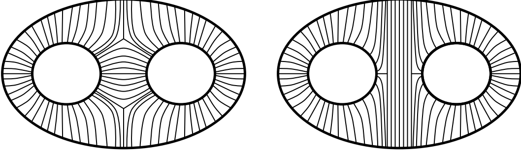
FIGURE 2. The two options for the foliation underlying an element of \mathcal{MF}_0(P) .
