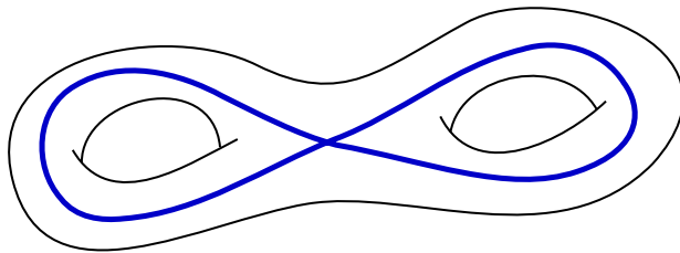
FIGURE 1. A closed curve with a single self intersection
