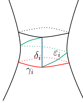
FIGURE 3. A pants curve \gamma_i and two arcs \delta_i and \varepsilon_i .
