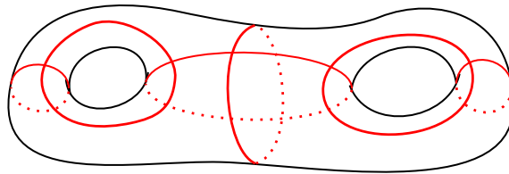
FIGURE 2. A filling collection of curves.
