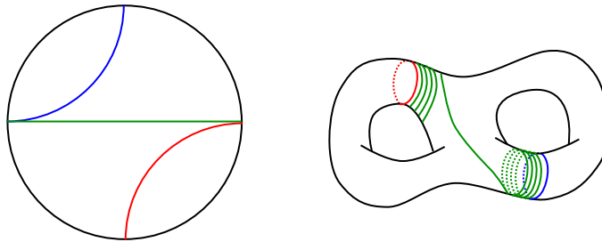
FIGURE 3. A lamination consisting of two simple closed geodesics and one geodesic arc. The left hand side consists of three lifts of the components to \mathbb{H}^2
