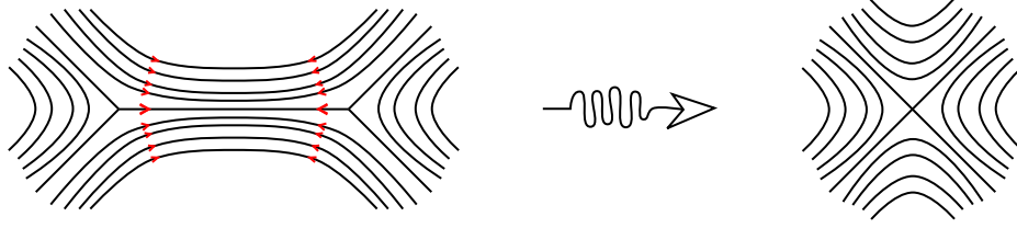
FIGURE 1. A Whitehead move, turning two 3-pronged singularities into a single 4-pronged singularity
