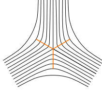
FIGURE 1. A full system of transversals near a three-pronged singularity.
