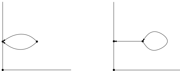
Figure 7 - The only two admissible graphs of type (1,2) appearing in \mathbb{A}_1
