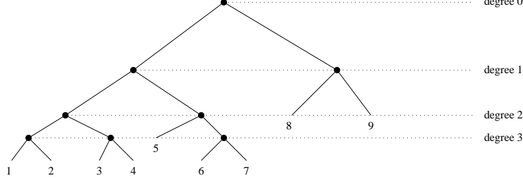
FIGURE 4. There are 8 nodes
