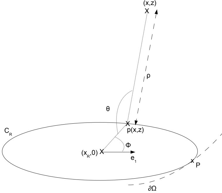
Figure 2: The coordinates (\rho, \theta, \phi) .
