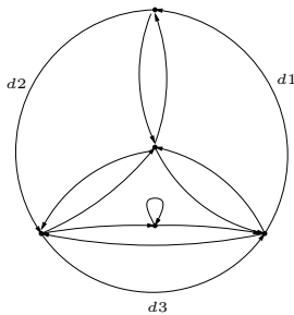
Figure 5: Block for cycle covers
