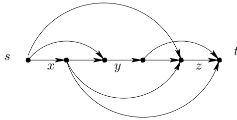
Figure 8: Block for s-t-paths
