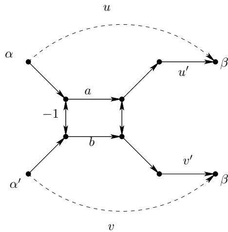
Figure 9: Iff gadget for s-t-paths
