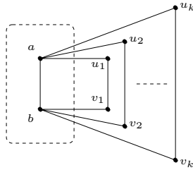
Figure 3: Couple for maximal independent set
