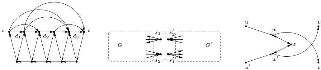
Figure 4: Block, Join and XOR for Hamiltonian cycles
