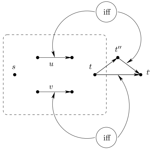
Figure 10: Couple for s-t paths
