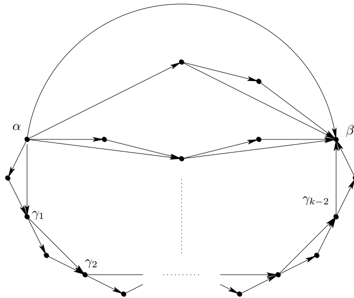
Figure 11: 2^k - 1 paths
