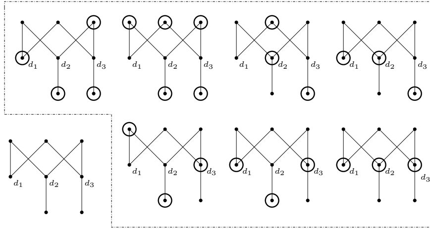
Figure 2: Block for maximal independent set and its solutions
