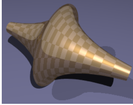
Figure 4.2. The pseudosphere is a surface in \mathbb{R}^3 isometric to the union of two truncated cusps, each with constant gaussian curvature -1 .
