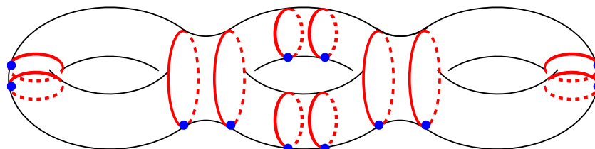
Figure 8.7. Decompose S into pairs of pants and annuli, so that each closed curve separates a pair of pants from an annulus. We fix a blue point in each curve.
