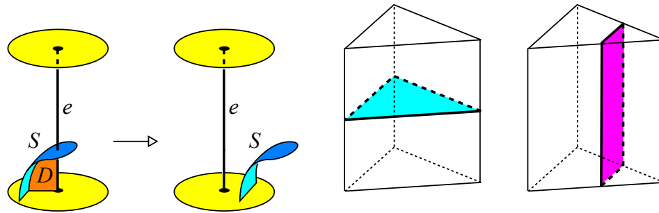
Figure 9.19. A move that decreases the intersection number of S with the vertical edges (left). The surface S intersects every prism into horizontal triangles (centre) or vertical rectangles (right).
