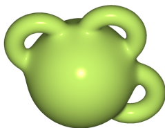
Figure 9.6. A handlebody of genus 3.
