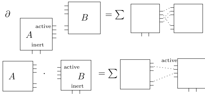
Figure 2: The operators \partial and \cdot .
