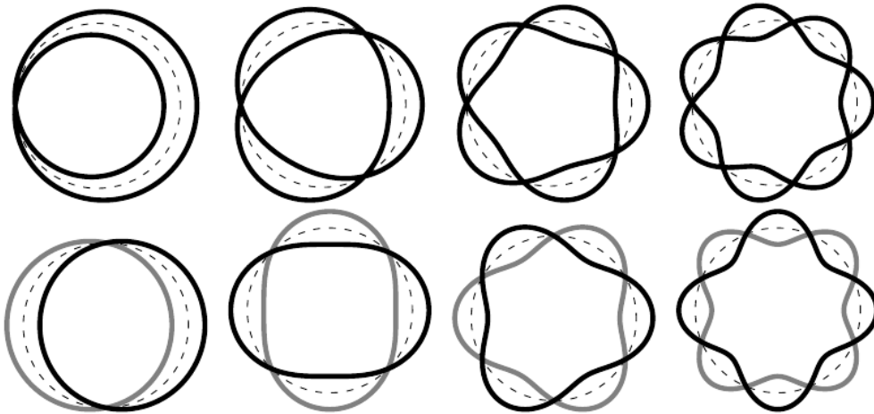
FIGURE 6. The simplest rank two Stokes diagrams.
