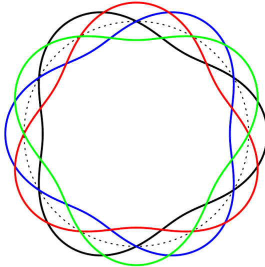
FIGURE 8. Example rank four Stokes diagram.
