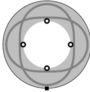
FIGURE 9. \Sigma = (\mathbb{P}^1, \infty, \Theta) , \Theta = n\langle x^2 \rangle + m\langle -x^2 \rangle .
