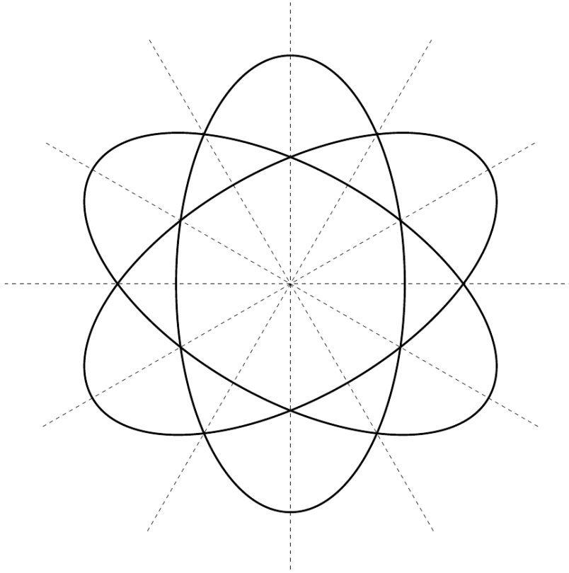
FIGURE 7. Example rank three Stokes diagram.
