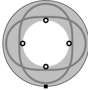
FIGURE 10. \Sigma = (\mathbb{P}^1, \infty, \Theta) , \Theta = n\langle x^2 \rangle + m\langle -x^2 \rangle .
