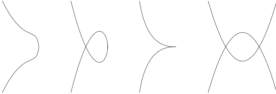
Figure 3 Examples of spectral curve
