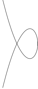
Figure 2 A projective line with a node
