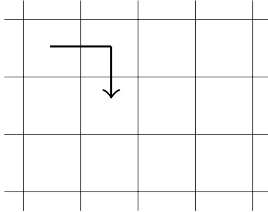
Figure 4 A product of two infinite chains of \mathbb{P}^1 In bold the action of \mathbb{Z}
