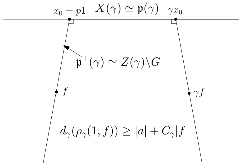
FIGURE 1. Normal coordinate
